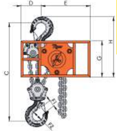
10t fishtail
