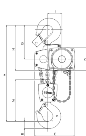
Triple Reeved
